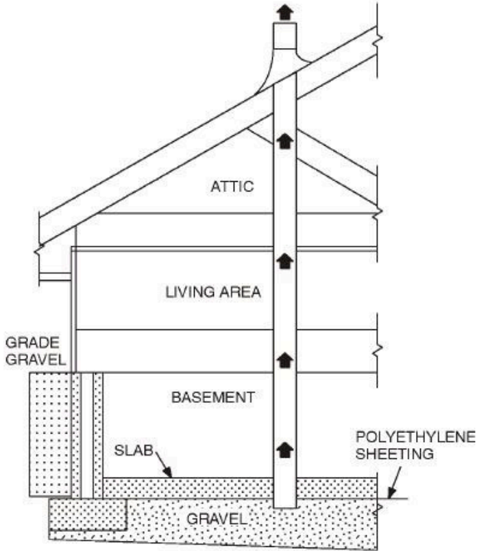
TYPICAL SUB-SLAB DEPRESSURIZATION PASSIVE RADON SYSTEM
