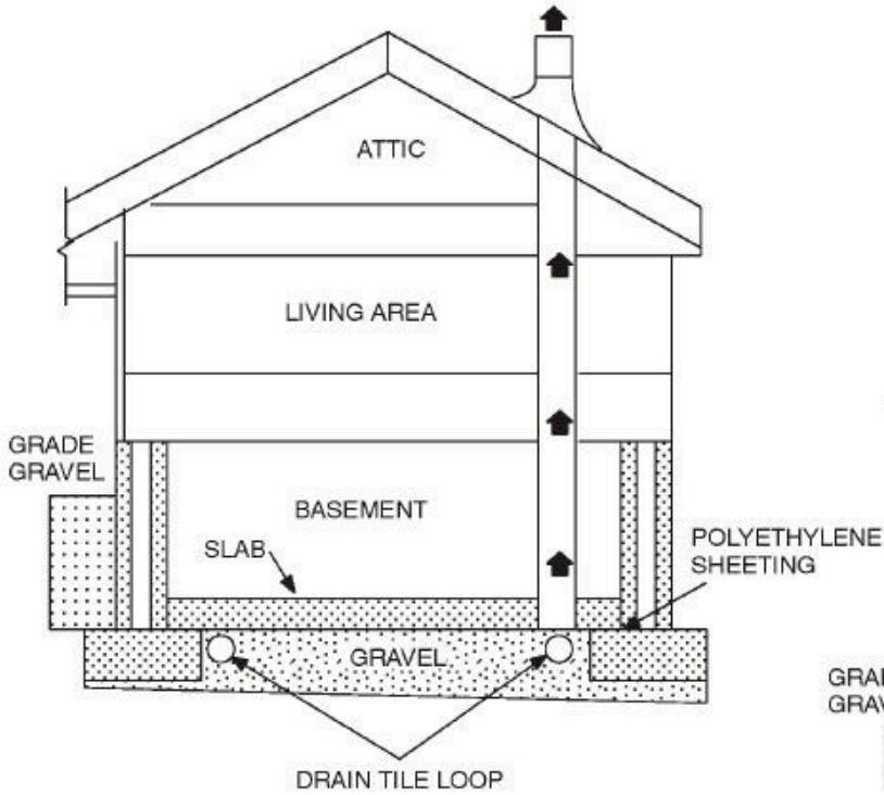
PASSIVE RADON SYSTEM USING DRAIN-TILE LOOP
