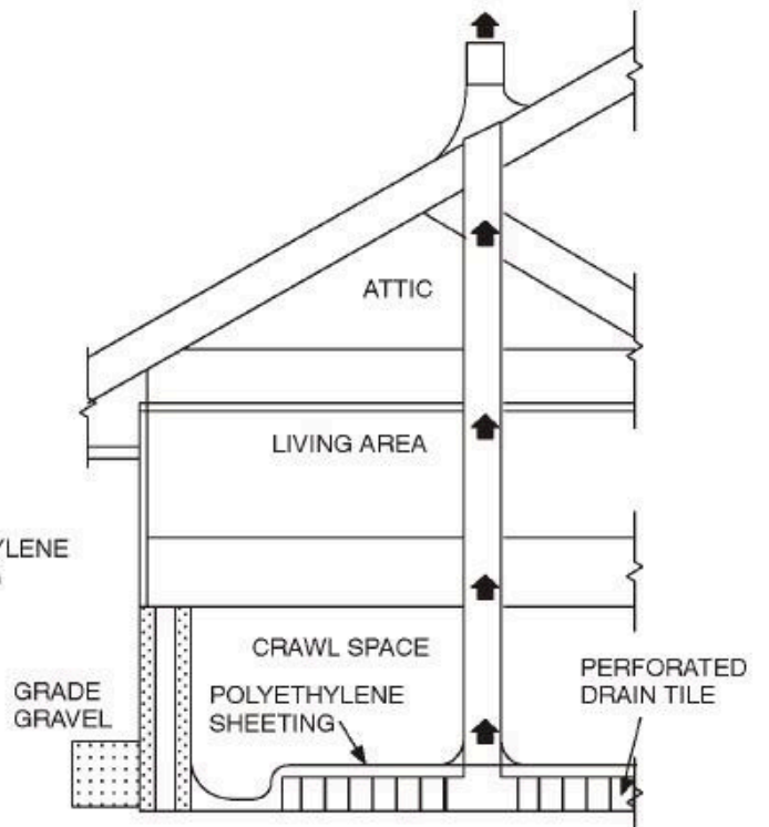
SUB-MEMBRANE DEPRESSURIZATION SYSTEM FOR CRAWL SPACE
