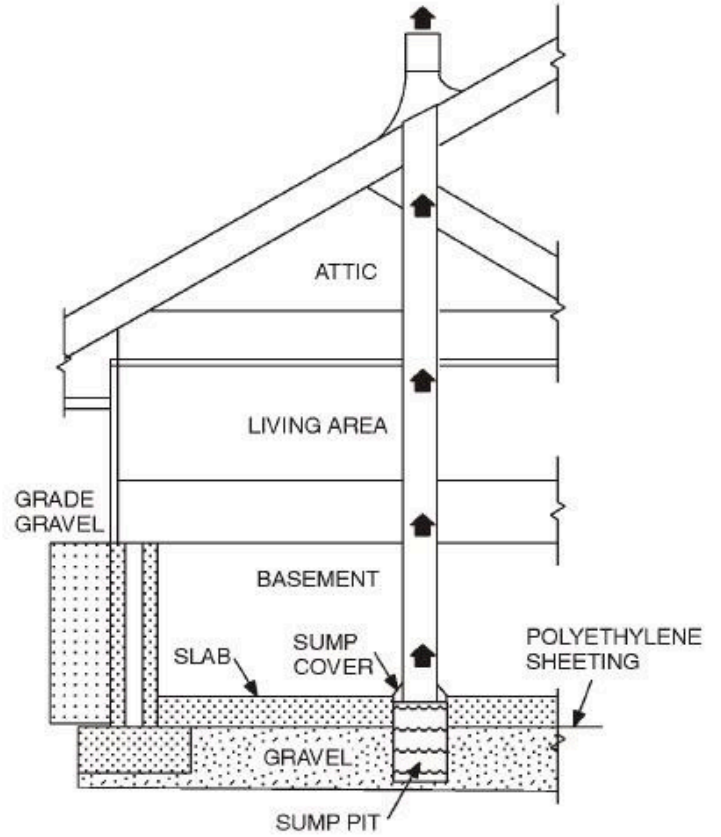
PASSIVE RADON SYSTEM VENTED THROUGH SUMP
